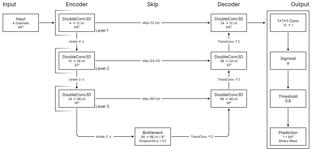
Figure 5.4: Phase I Final U-Net Architecture
