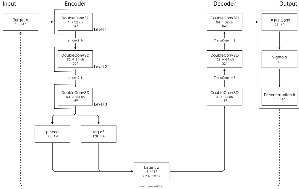
Figure 5.17: Phase III Stage A Reference VAE Architecture
